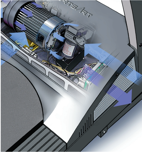
FlowTec™ motor system: Cools and cleans motor for better performance and longer life
